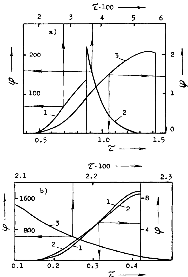
FIGURE 2 Normalized to unity relaxation time spectra for prolate (a) and oblate (b) particles.
