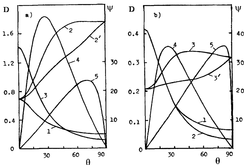
FIGURE 1 Angular dependence of the selfdiffusion tensor for prolate (a) and oblate (b) particles.
